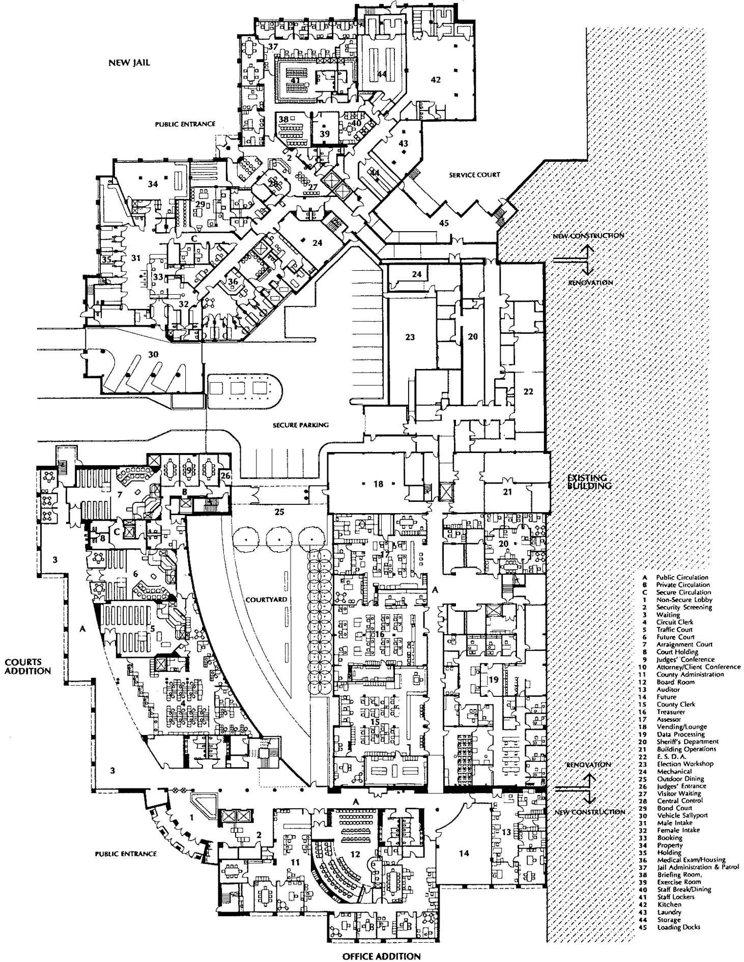
FIRST FLOOR 0 5 10 20 40 FEET
